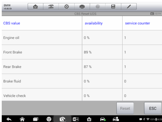
Figure 5-3 Sample Oil Reset Service Screen 2
